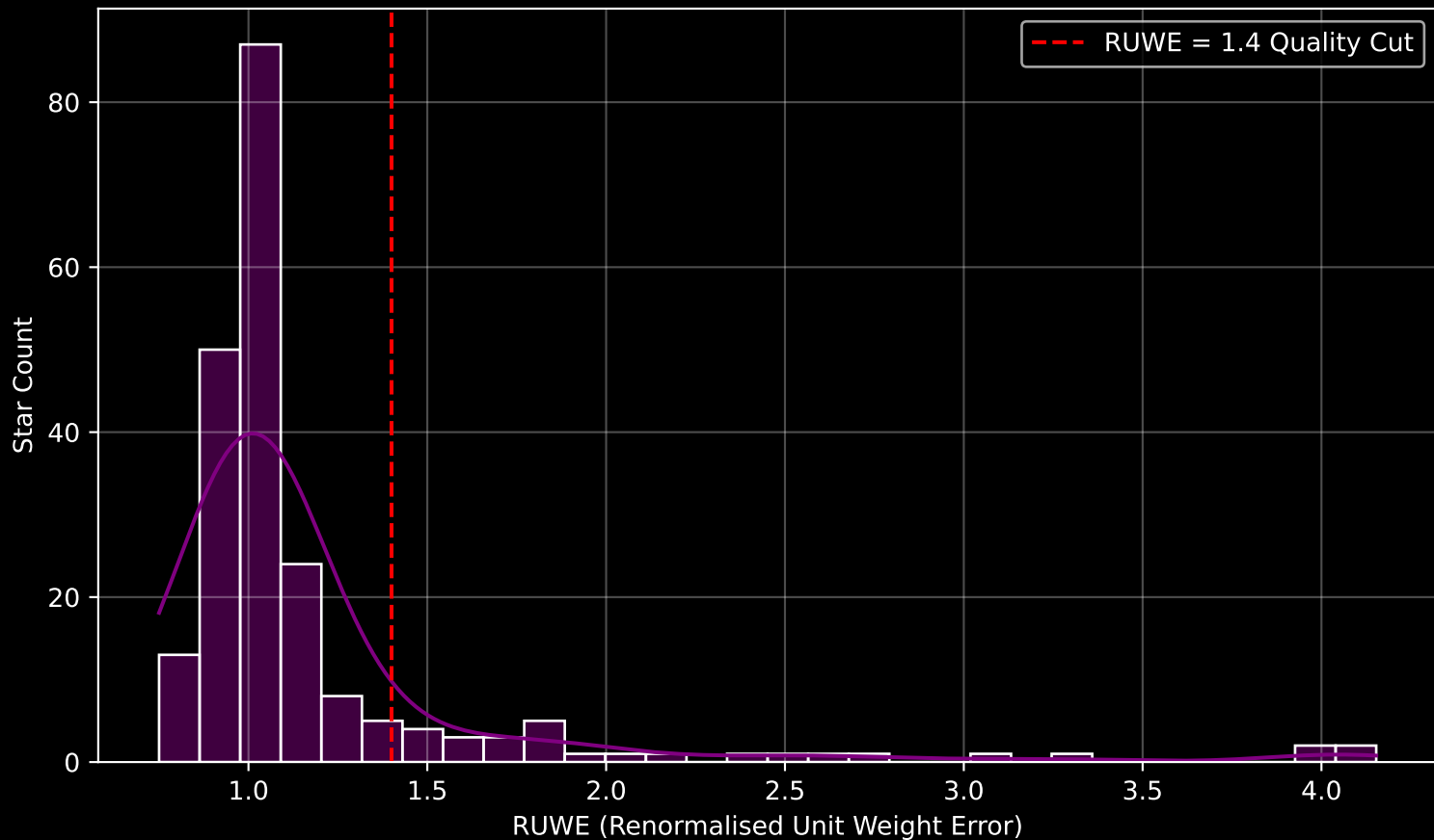
GAPOGEE DR17 Field [049-52-O] RUWE Distribution (n= 215)
