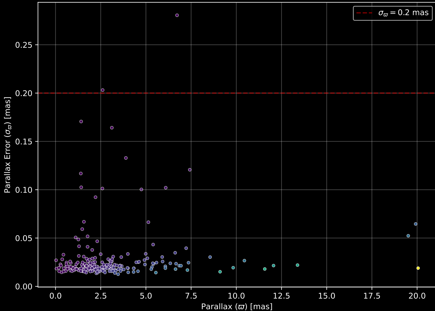
APOGEE DR17 Field: [049-52-O] Parallax Quality (n= 225)
