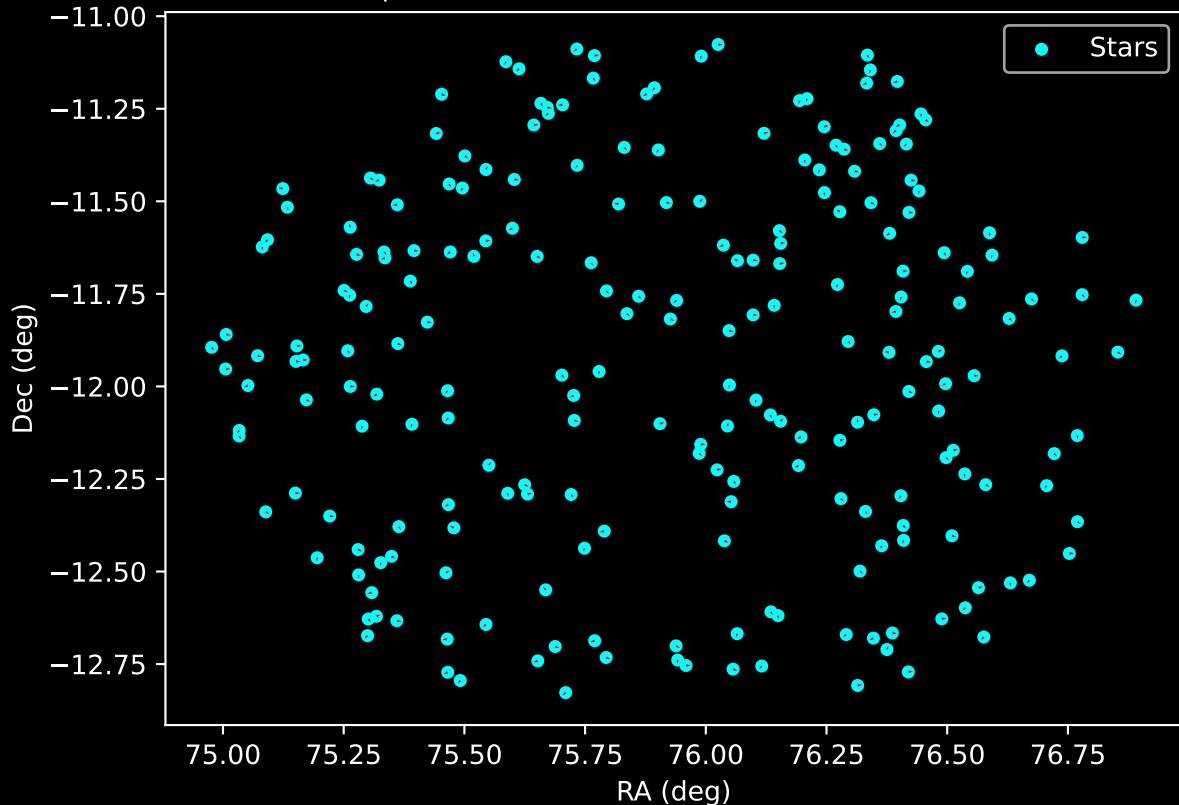
APOGEE DR17 Field: [049-52-O] Proper Motion Vectors for Gaia Star Field (n= 225)
