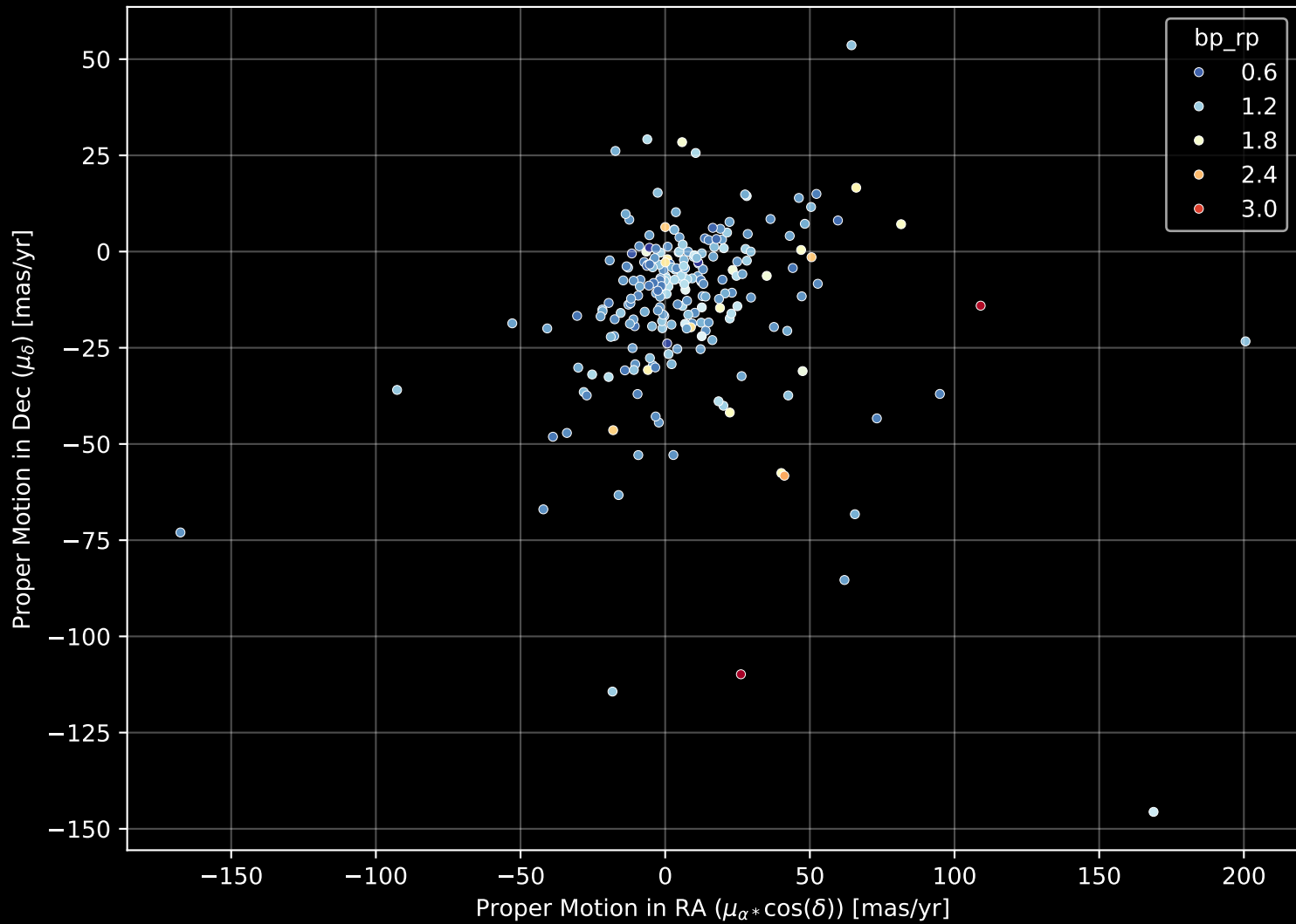
APOGEE DR17 Field: [049-52-O] Proper Motion Diagram (n= 225)
