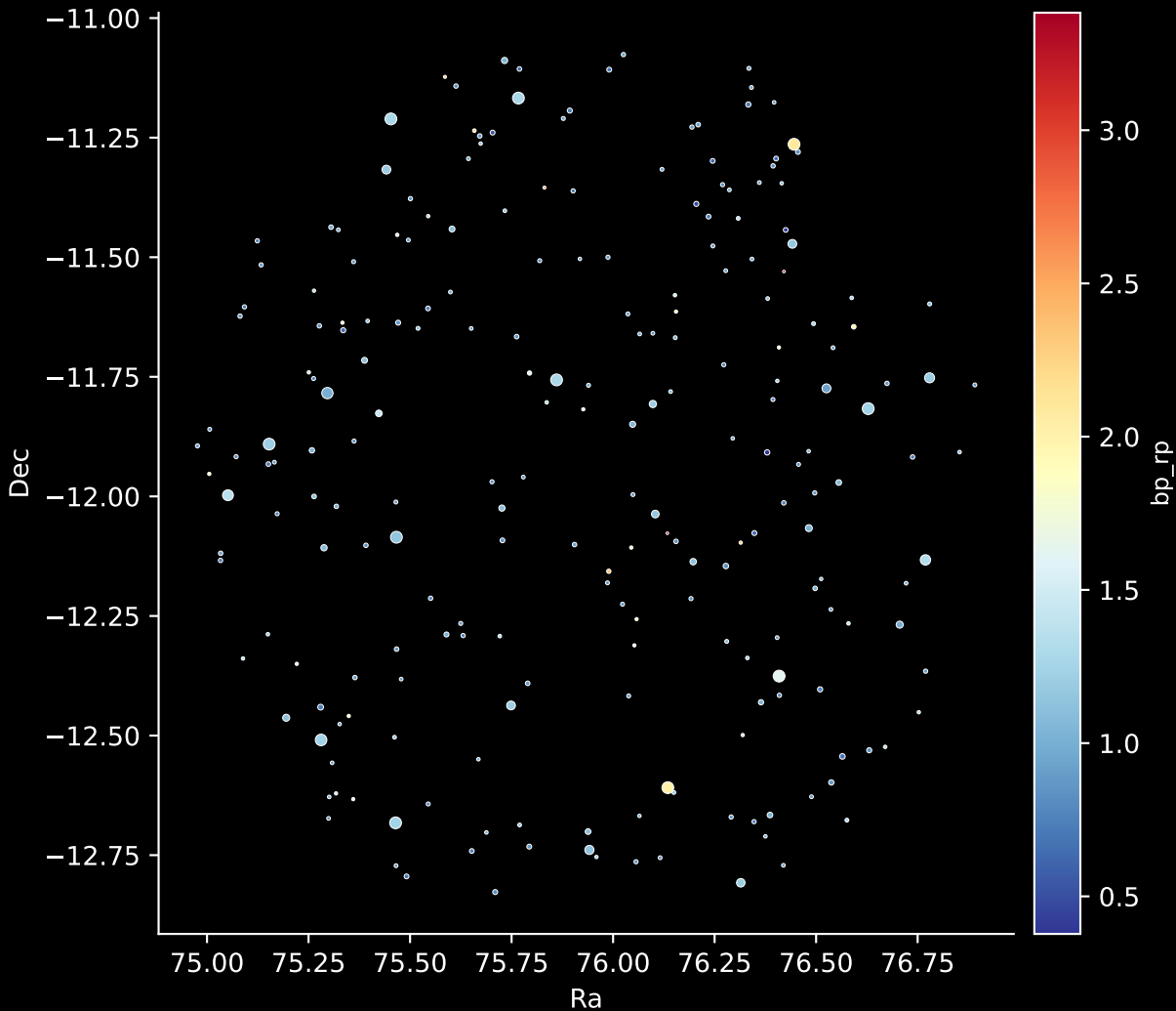
APOGEE DR17 Field: [049-52-O] Stars: 225
