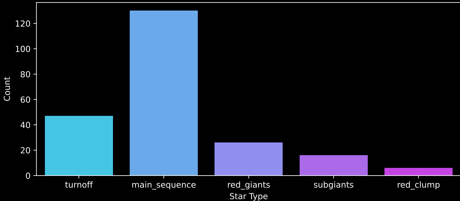
APOGEE DR17 Field: [049-52-O] Count plot of Star Type
