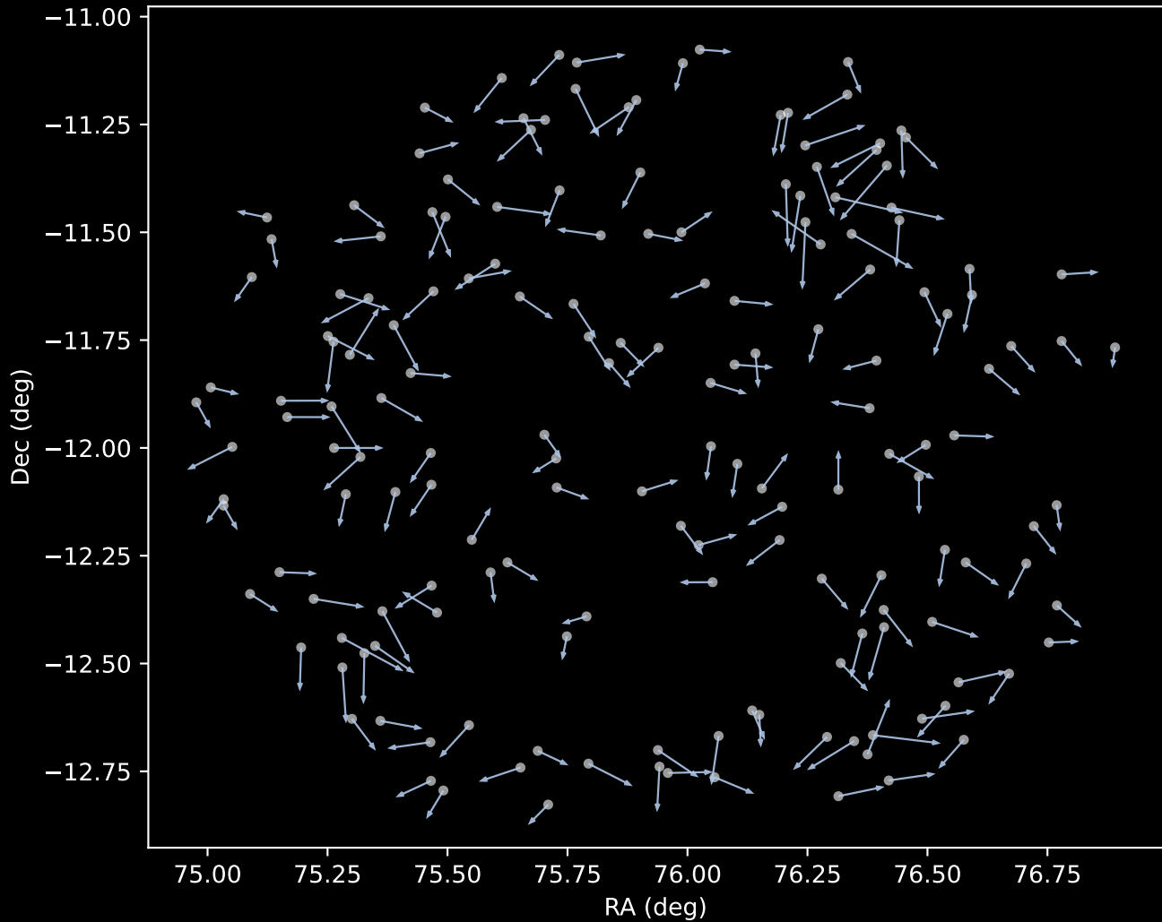
APOGEE DR17 Cluster 1 Proper Motion Vectors (n=170)
