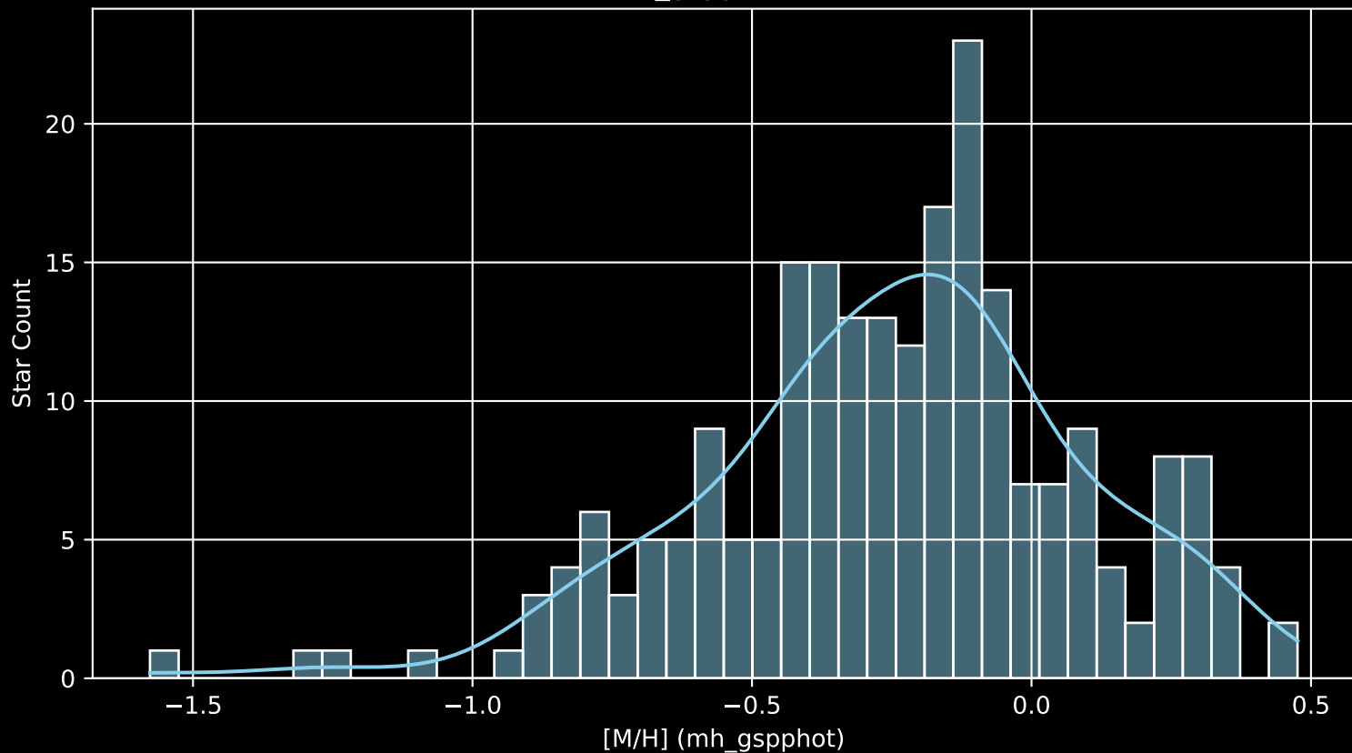
APOGEE DR17 Field: [049-52-O [M/H] (mh_gspphot) (n= 223)
